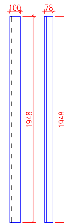
AT BLENDA 1KS DTD-L H1277 akacie/abs 2mm
